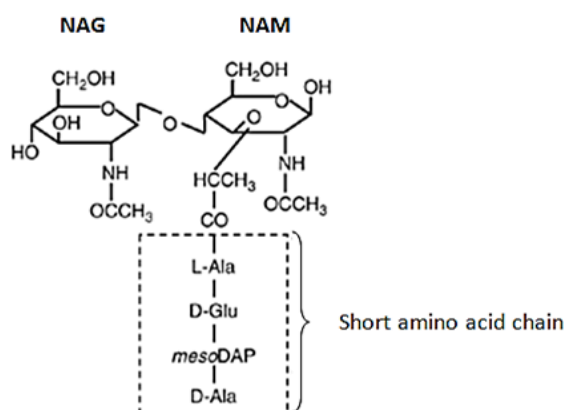
molecular structure of NAG and NAM
